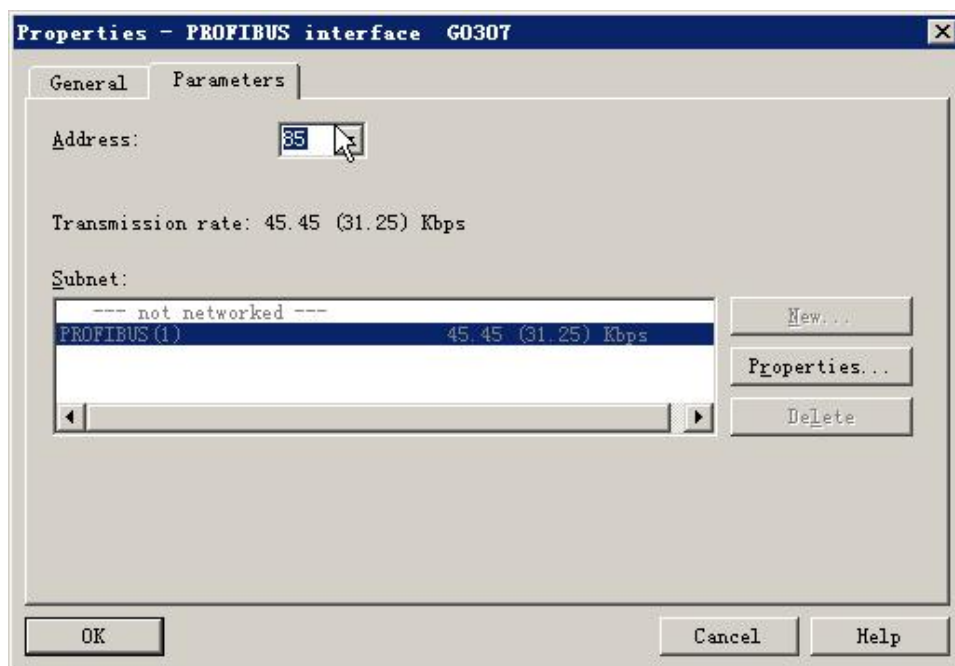
Figure 14 Device Prosperities Configuration
