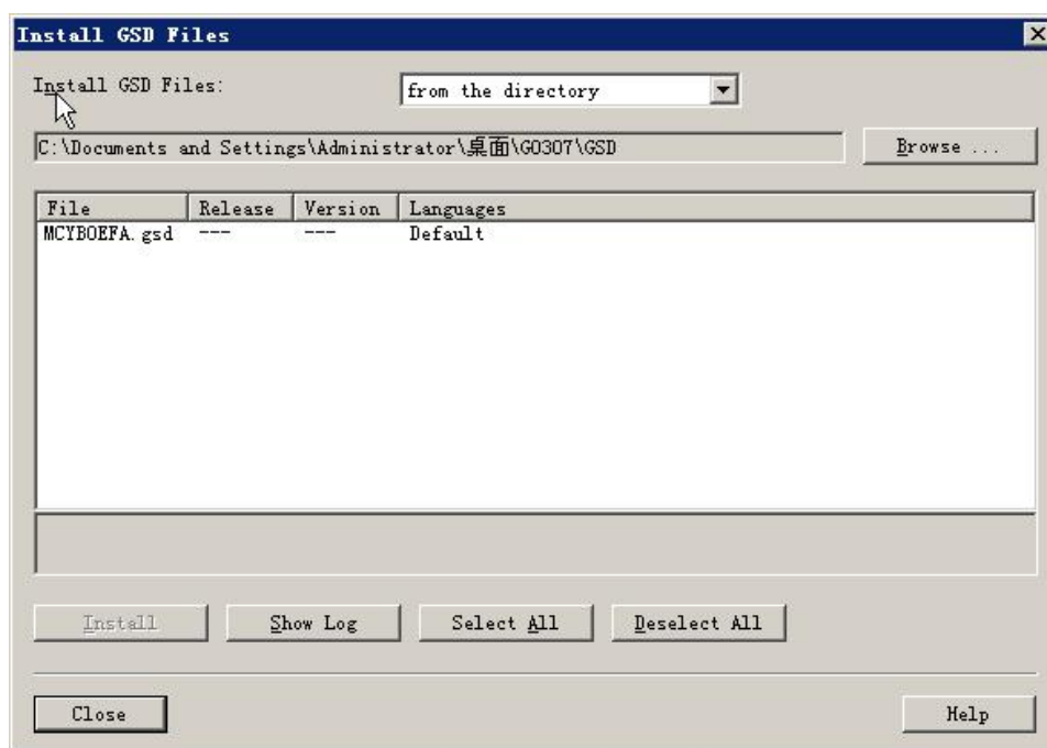
Figure 11 GSD File Window
